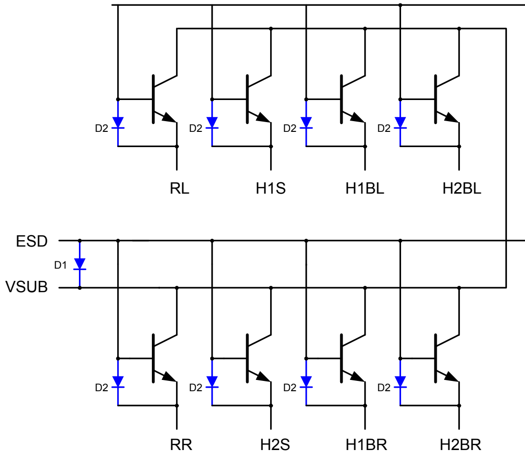
Figure 2: ESD Protection
