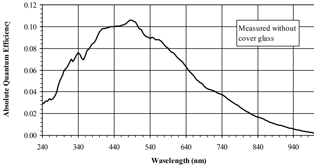
Figure 7: Monochrome Quantum Efficiency
