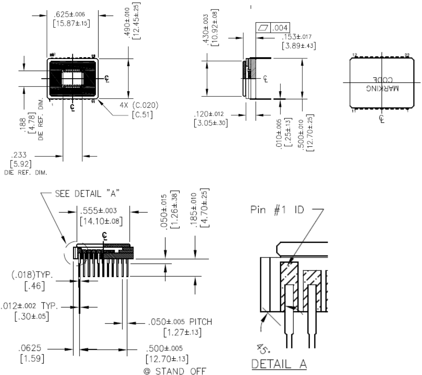
Figure 20: Package Drawing
