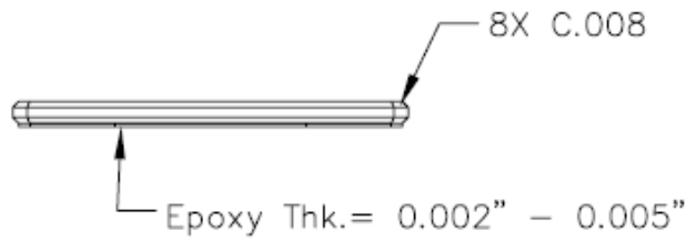
Figure 22: Glass Drawing
