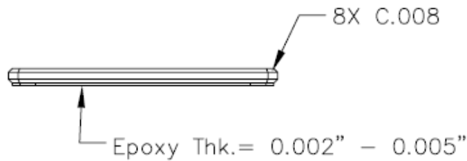
Figure 23: Quartz Cover Glass
