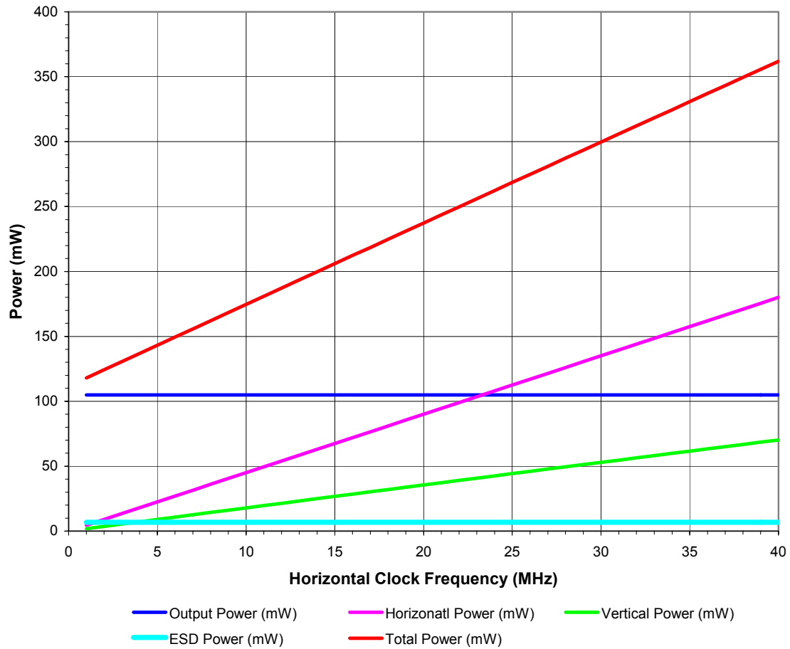
Figure 3: Power
