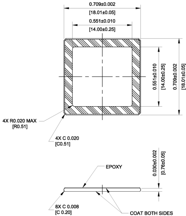
Figure 26: PGA Cover Glass
