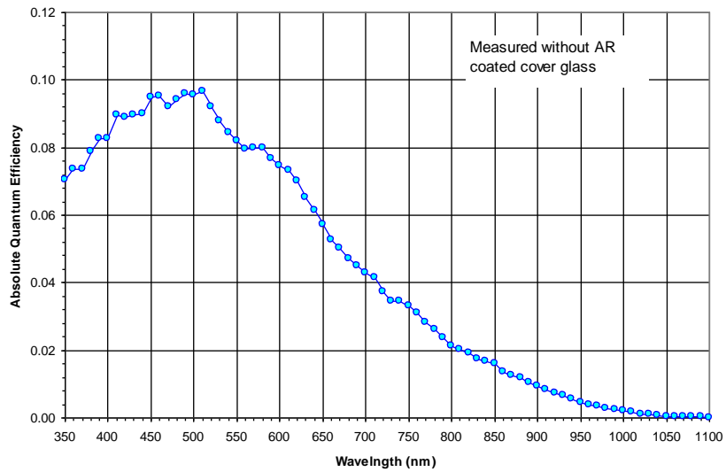
Figure 7: Monochrome without Microlens Quantum Efficiency
