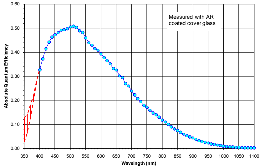
Figure 6: Monochrome with Microlens Quantum Efficiency
