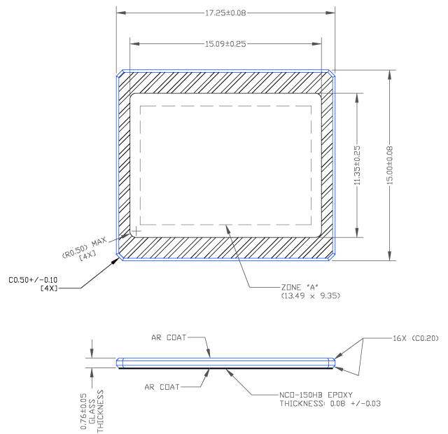
Figure 27: CLCC Cover Glass
