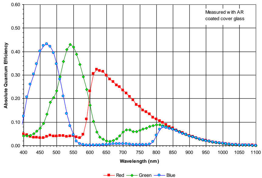
Figure 4: Color with Microlens Quantum Efficiency
