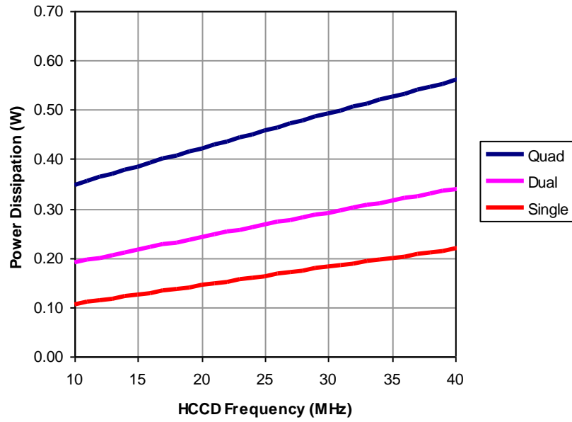
Figure 7: Power
