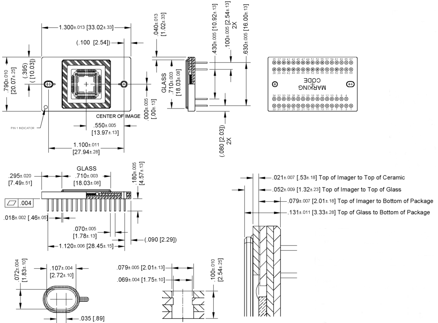
Figure 20: Completed Assembly
