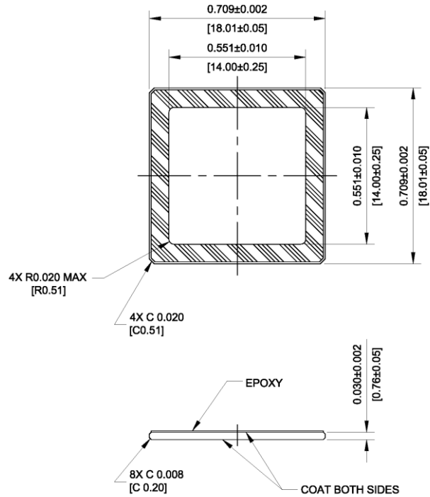
Figure 21: Cover Glass
