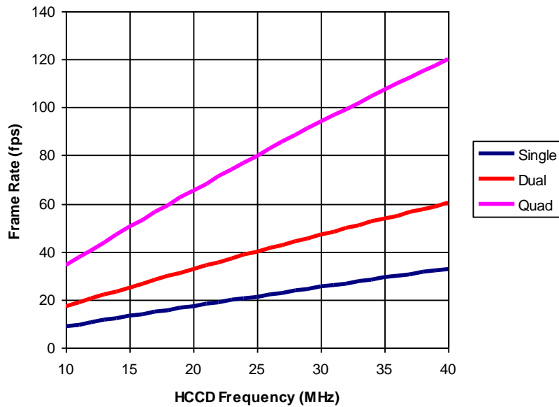
Figure 8: Frame Rates
