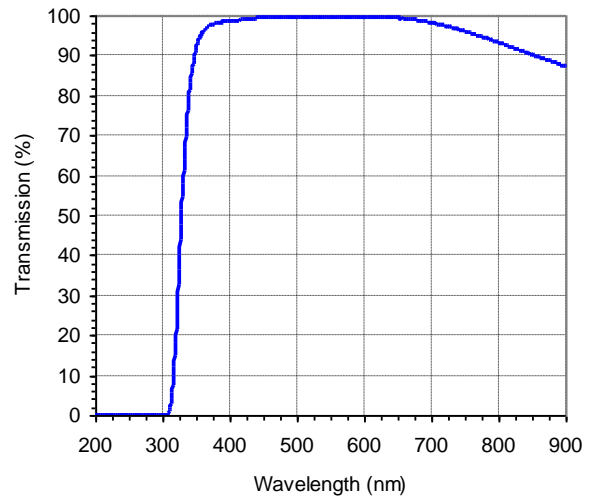
Figure 22: Cover Glass Transmission
